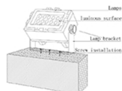
Installation Illustration
