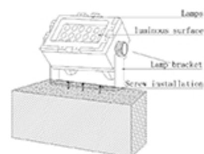
Installation Illustration
