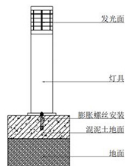
Installation Illustration
