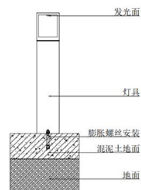
Installation Illustration
