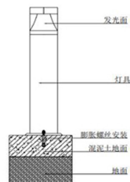
Installation Illustration
